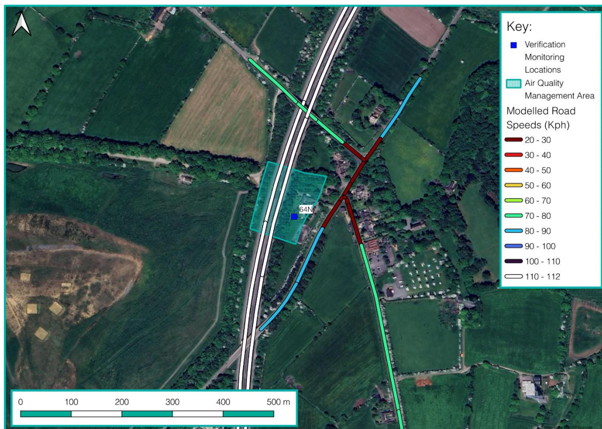
Figure 8a.10: Location of Verification Monitoring Location (Verification 10)
