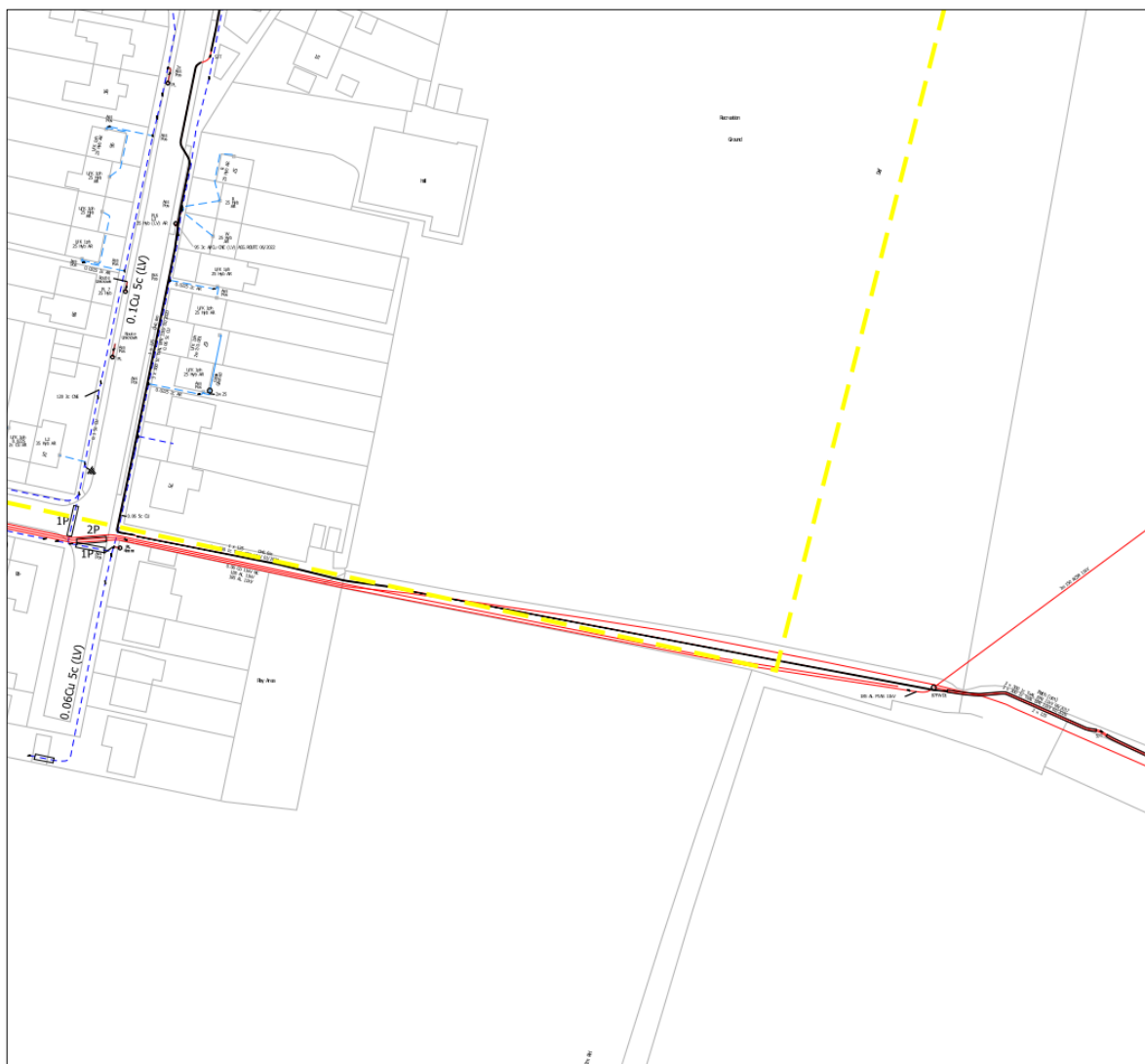
Figure 5.15.1 – Existing underground 11kV (HV) cables running along the existing public footpath
