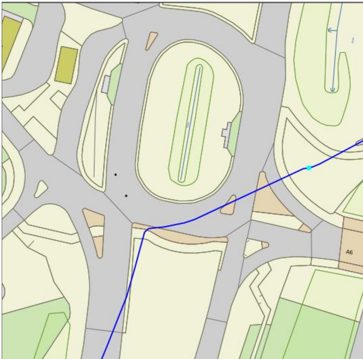
Figure 5.11.11 – Existing underground ducts and chambers within and in close proximity to the existing roundabout
